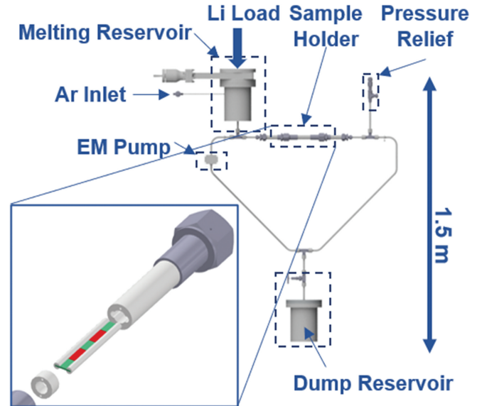
Fig. 11. Proposed corrosion loop to test different materials under flowing lithium conditions. This will be done in an argon atmosphere for simplicity.
