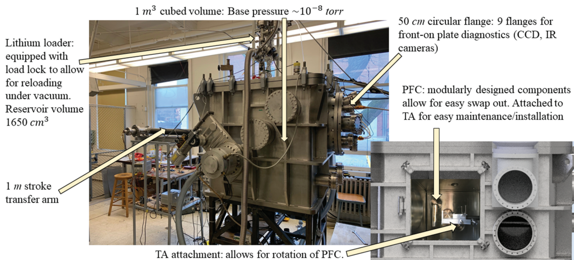
Fig. 1. The MEME system used on EAST is designed to develop plug-and-play LM systems for EAST. Currently, it is being used to develop LM loops and wetting experiments for the LMPFC program.
