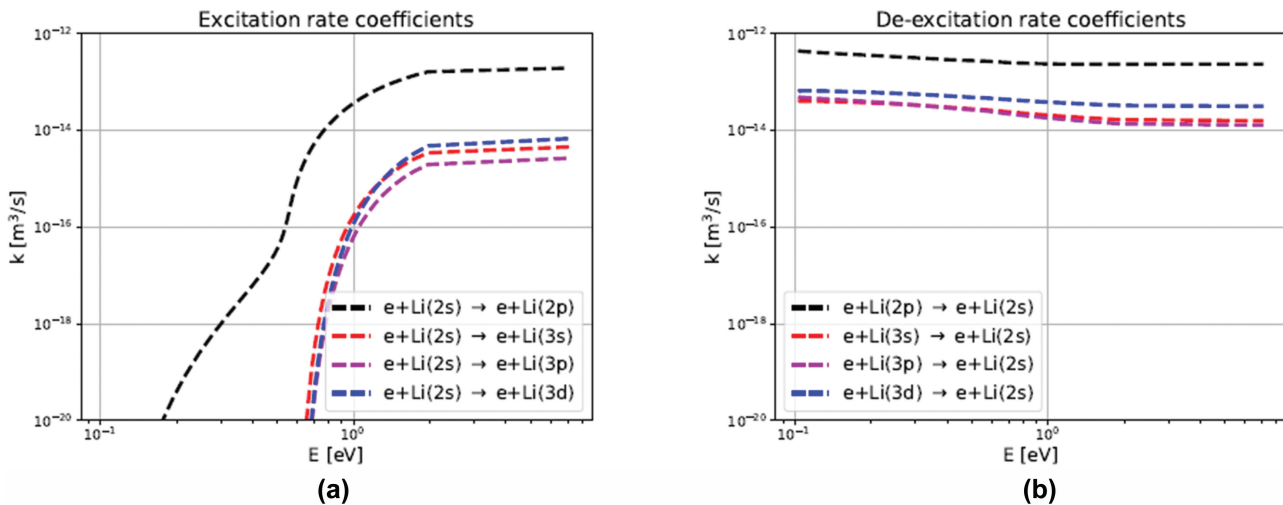
Fig. 9. (a) Excitation and (b) deexcitation rates for lithium species. This shows that the deexcitation reaction rates are much higher than the excitation ones.
