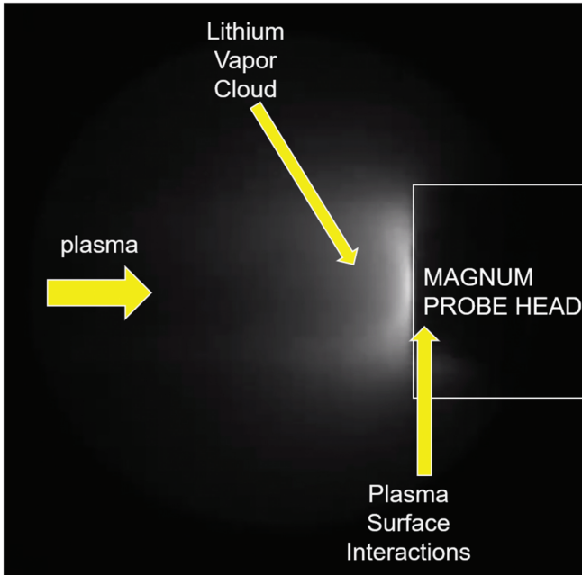
Fig. 7. Image showing where the MAGNUM-PSI probe head is with plasma surface interactions and where the lithium vapor cloud occurs. The plasma is coming in from left to right.
