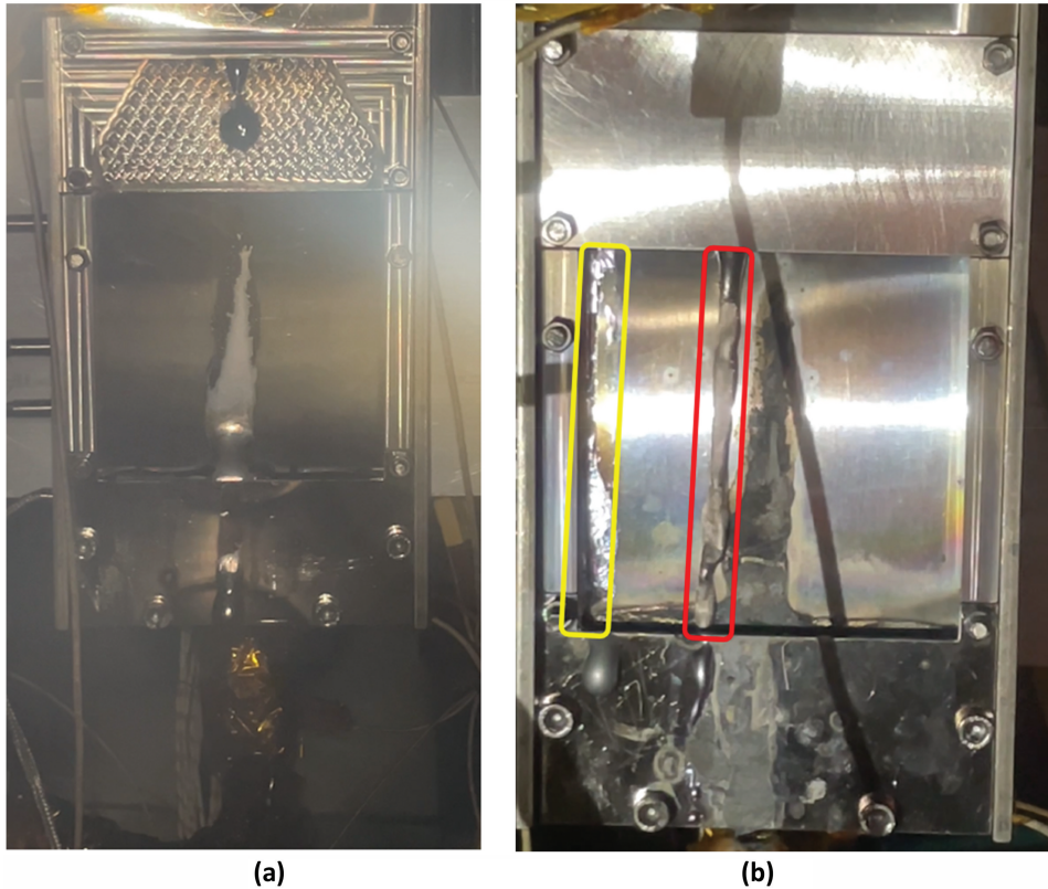
Fig. 4. (a) Initial loop and distributor tests in the MEME showing that when lithium gets on the stainless steel plate there is wetting. The distributor posts are clearly seen. (b) The cover plate is now installed, and a clear stream of flowing liquid lithium is flowing down the plate.
