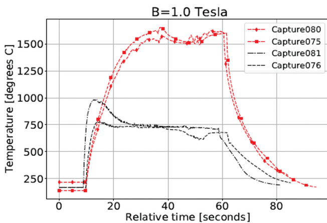
Fig. 6. Example of the LVS: 15 to 20 MW·m -2 heat flux discharges without lithium (red) and with lithium (black) where the locking temperature is clearly observed.
