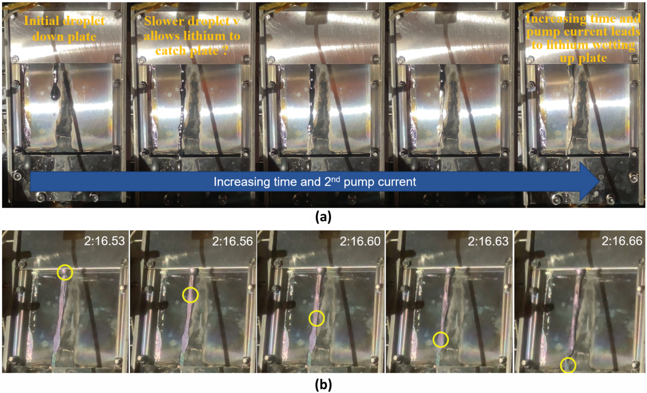
Fig. 5. (a) Changes in the flow of the lithium with increasing EM pump current, going from drops to an unstable flow to a stable laminar flow. (b) The flow velocity is estimated by looking at a bulge feature that travels down the flow and is measured to be 1 m/s.
