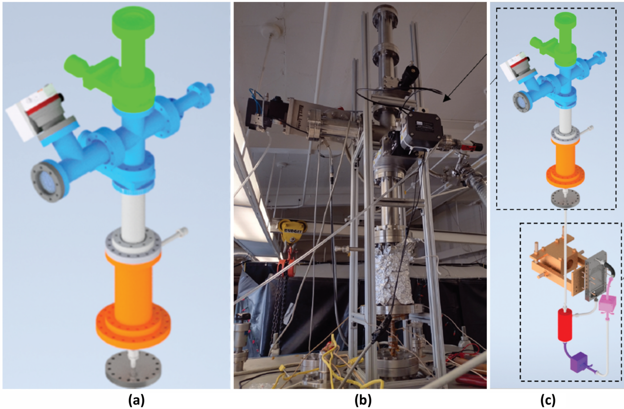
Fig. 3. (a) CAD drawing of the lithium loading system that is used to load lithium into the lithium loop on the MEME. A suitcase (green) has the lithium loaded in a glove box filled with argon. This then attaches to an evacuation system (blue) where the argon is pumped out and the lithium is pumped to low pressures to minimize the amount of tarnishing of the lithium. This is then dropped into a premelting reservoir (orange) where the lithium is melted and then flows through a pipe into the internal reservoir of the loop. (b) Photo of the lithium loading system on the MEME. (c) CAD drawing showing the lithium loading system connected to the lithium loop system.
