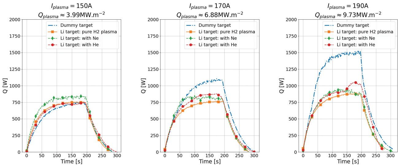
Fig. 8. Heat flux measurements of plasmas on the surface of the MAGNUM-PSI. Four separate experiments were done for each value of heat flux. The first (blue) is a nonlithium plasma, the second (orange) is lithium with just hydrogen, the third (green) is lithium with neon, and finally, the fourth (red) is lithium with helium: (a) 3.99 \text{MW}\cdot\text{m}^{-2} , (b) 6.88 \text{MW}\cdot\text{m}^{-2} , and (c) 9.73 \text{MW}\cdot\text{m}^{-2} . It is clear to see that below a threshold of heat flux there is no effect, but above some value of heat flux what is seen by the surface is reduced and limited to about 5.5 \text{MW}\cdot\text{m}^{-2} .
