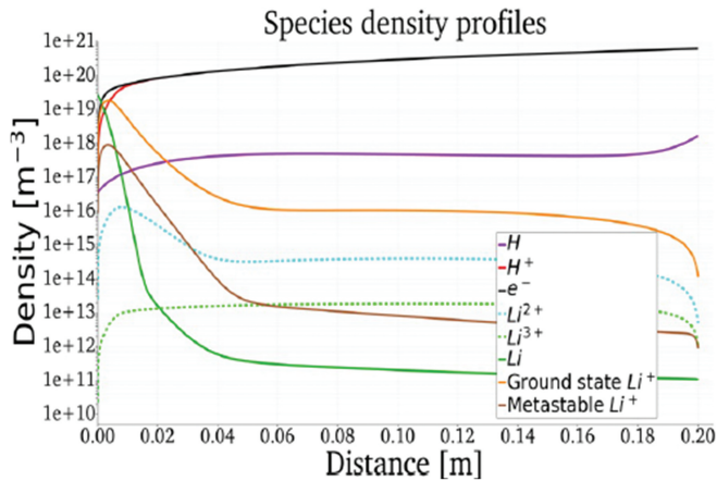
Fig. 10. Density profiles for different species within the vapor cloud. This not only includes the lithium species, but also incoming plasma.
