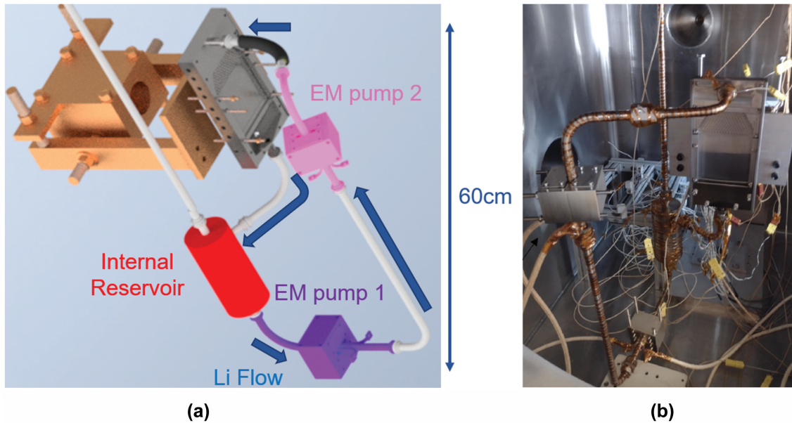
Fig. 2. (a) CAD drawing of the internal flowing liquid-lithium loop that is installed and being tested in the MEME for the program. The internal reservoir (red) has lithium loaded into it via an external loading system. Once the lithium melts and the system reaches 270°C, the lithium flows into the first EM LM pump (purple), which pumps the lithium up to the second EM LM pump (pink) and to the distributor and PFC plate (gray) system for wetting studies. The lithium is then collected and flows back to the internal reservoir, completing the whole loop. The system has been continuously run for several 10s of minutes at a time. (b) Actual photo of the internal loop inside the MEME.
