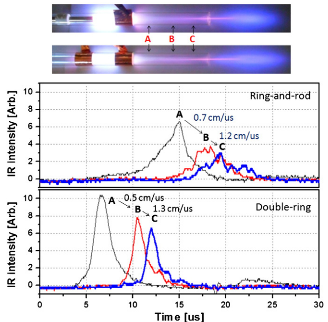
Fig. 6. Light emission profiles measured at 2 cm, 4 cm and 6 cm away from the main discharge region.
