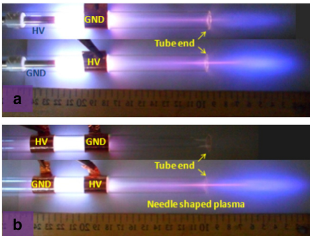
Fig. 2. Atmospheric pressure helium plasma from ring-and-rod (a) and double-ring structures (b).
