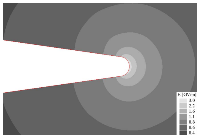
FIG. 3. (Color online) 2D simulation of the field distribution near the apex of the tip, illustrating the fast drop of electric field strength away from the point of maximum electric field.
